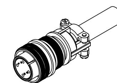
AIR-SIDE CONNECTOR
